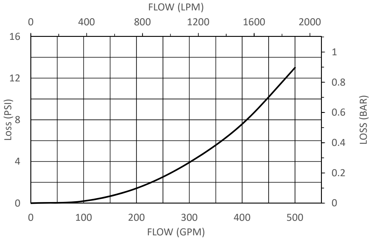
Figure B.1- Pressure loss chart
